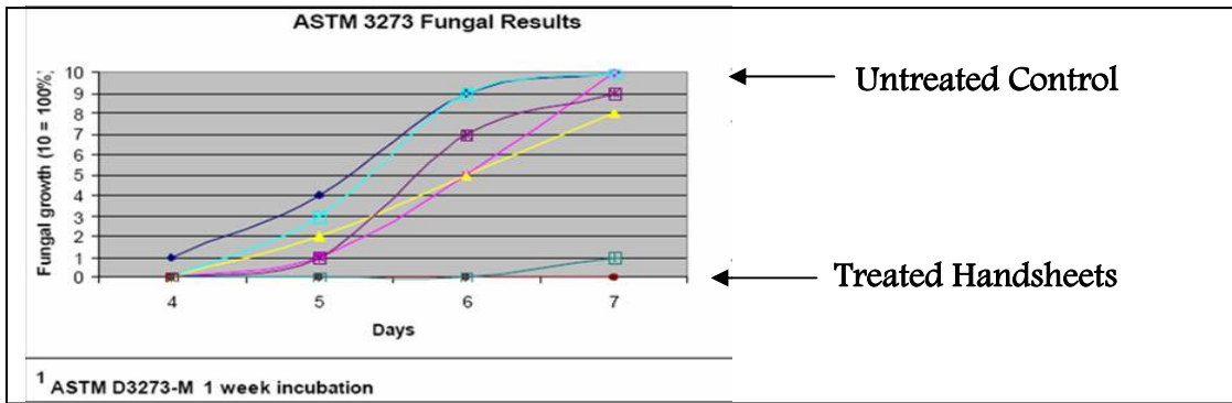
Fig 2. Percentage reading of fungal growth on untreated and treated wallboard.
